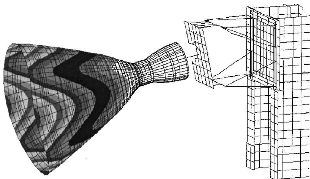
Fig. 5 Two ND mode of nozzle on test stand.
