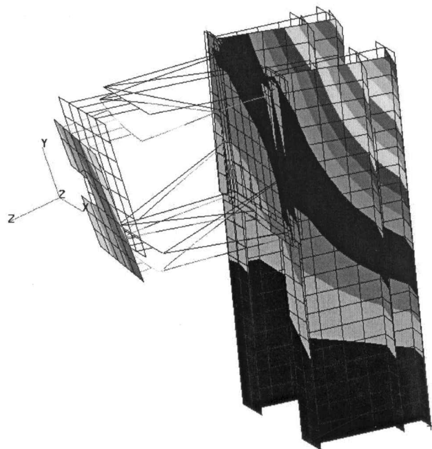
Fig. 3 Test stand, mode 2 at 50 Hz (deformed shape superimposed on undeformed shape).
