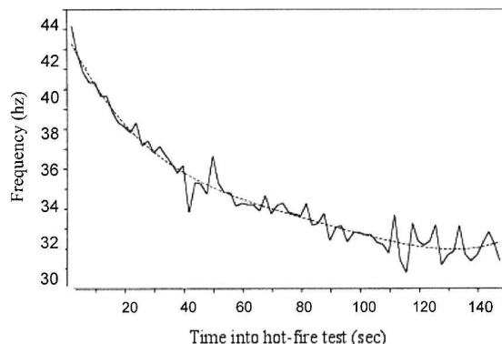
Fig. 6 Isolated time history trace of two ND mode frequency peak for accelerometer 11.
