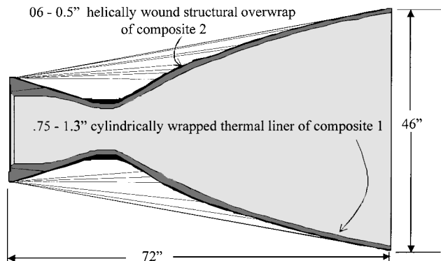
Fig. 1 Cutaway of X-34 FASTRAC rocket nozzle.
