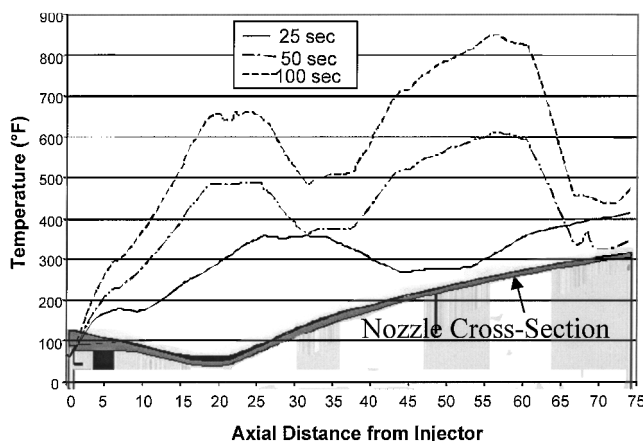
Fig. 7 Temperature of nozzle for various times into hot-fire test vs axial location.
