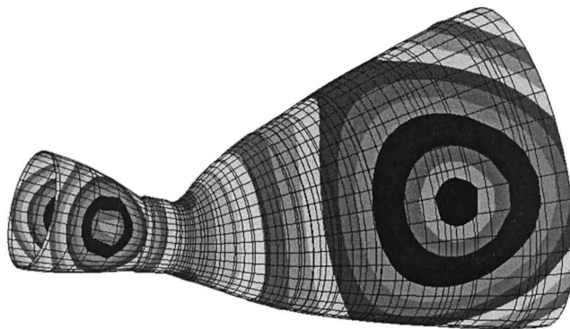
Fig. 4 Nozzle, free-free, first bending at 180.9 Hz.
