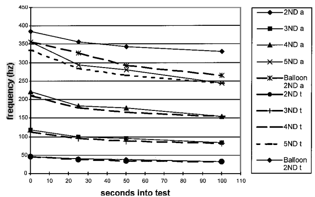
Fig. 8 Comparison of variation in natural frequencies vs time into hot fire between test and correlated analytical results.
