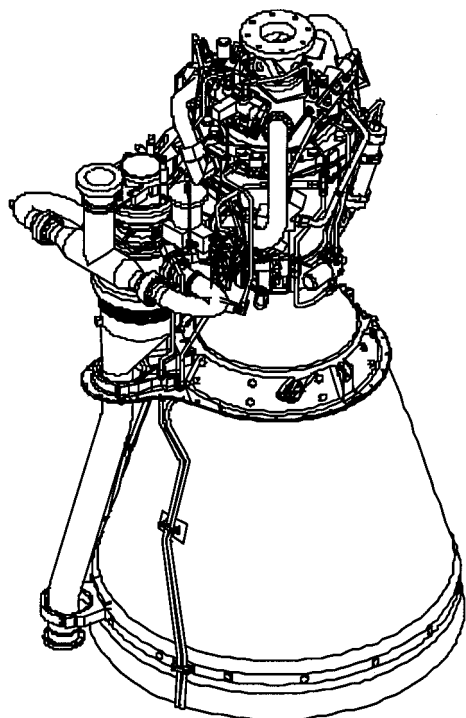
Fig. 2 Turbopump and other FASTRAC components mounted on nozzle.
